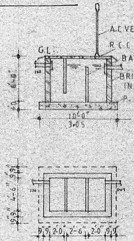
PLAN & SEC. OF SEPTIC TANK
